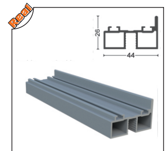
PRGLD-1004 Küçük h Fitiil Contalı Aluminum Small 'h' Seal(With PVC Seal)
