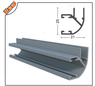
ALMFTL-1004 90° Fitil 90° Seal
