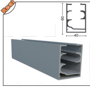
GLDPLS-1001 Kasa Profili Frame Profile
