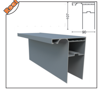
PRGLD-1003 Perdelik Ayak Profili Aluminum Curtain Profile
