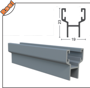
ALMFTL-1002 Büyük H Fitil Big H Seal
