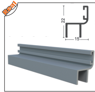
ALMFTL-1001 Küçük h Fitil Small h Seal
