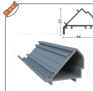
ISICM31-1015 135° Fitiil Aluminum 135° Seal
