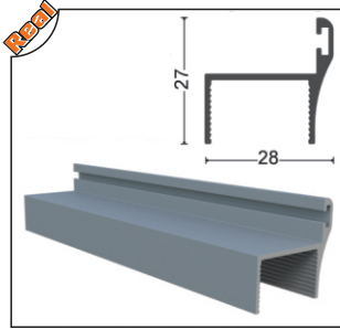
ISICM21-1004 Küçük h Fitiil Small "h" Aluminum Seal
