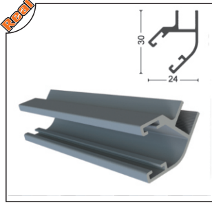
ALMFTL-1003 135° Fitol 135° Seal
