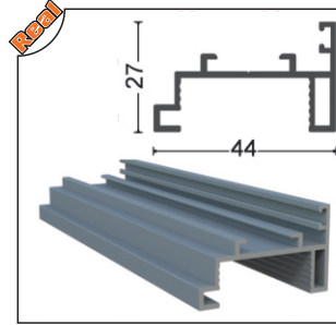
PRGLD-1006 Kollu Fitol Karşılığı Contalı Esp.Handle Opposite Alm. Seal (With PVC Seal)
