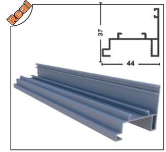
ISICM31-1017 İspanyolet Kollu Profili Espagnolette Arm Profile Of Opposite
