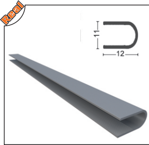
ALMFTL-1005 D Fitiil Aluminum "D" Seal
