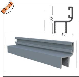
ALMFTL-1001 Küçük h Fitol Small 'h' Aluminum Seal
