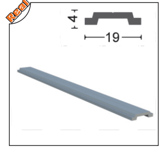
ISICM31-1013 Tij Profili Push Rod Profile
