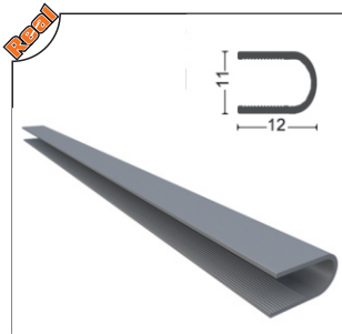
ALMFTL-1005 D Fitol Aluminum 'D' Seal
