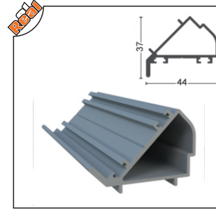
ISICM31-1015 135° Fitol Aluminum 135° Seal
