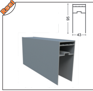
GLD-1005 Perdelik Ayar Profili Aluminum Curtain Profile
