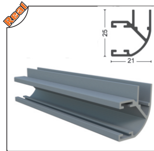
ALMFTL-1004 90 Fitol Aluminum 90 Seal
