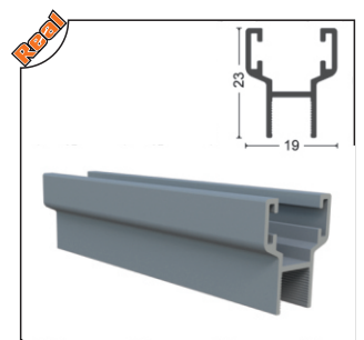
ALMFTL-1002 Büyük H Fitol Big 'H' Aluminum Seal
