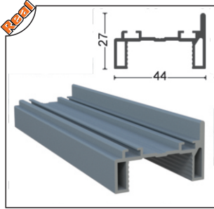
ISICM31-1010 Küçük h Fitol Contalı Esp.Handle Seal (With PVC Seal)
