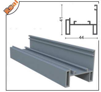
ISICM31-1001 Kollu Fitol Contalı Esp. Handle Alm. Seal(With PVC Seal)
